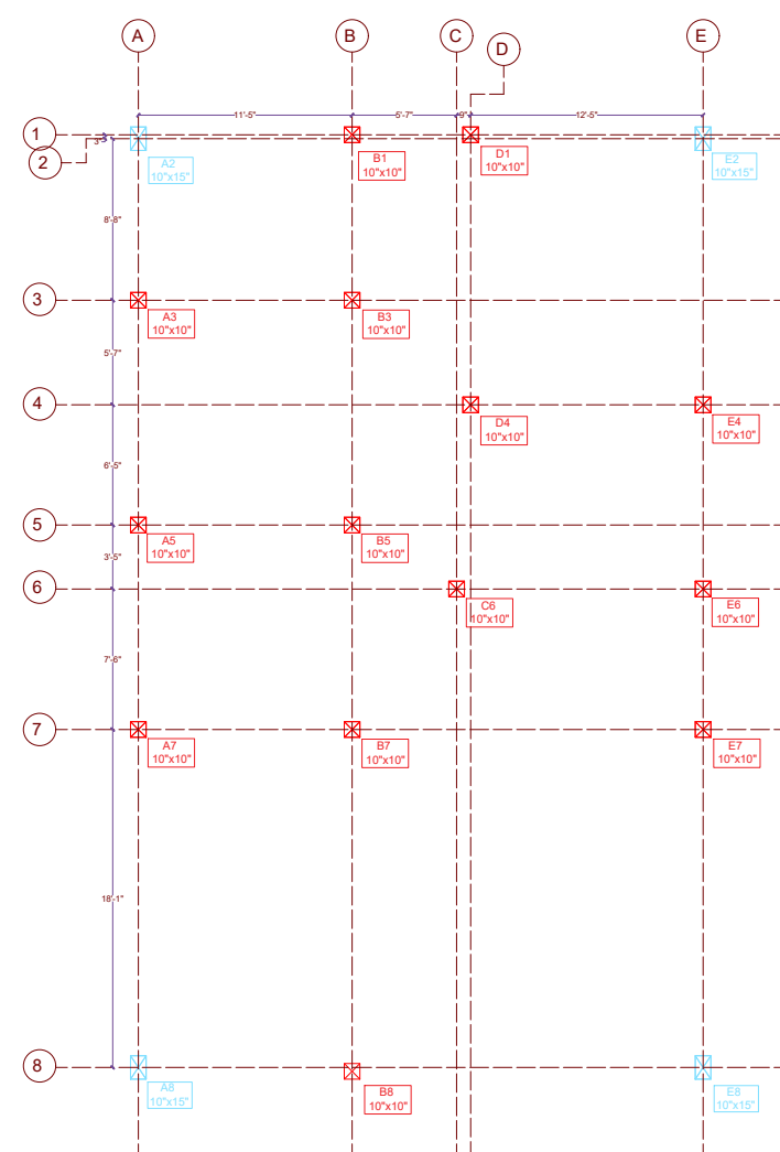
COLUMN LAYOUT
